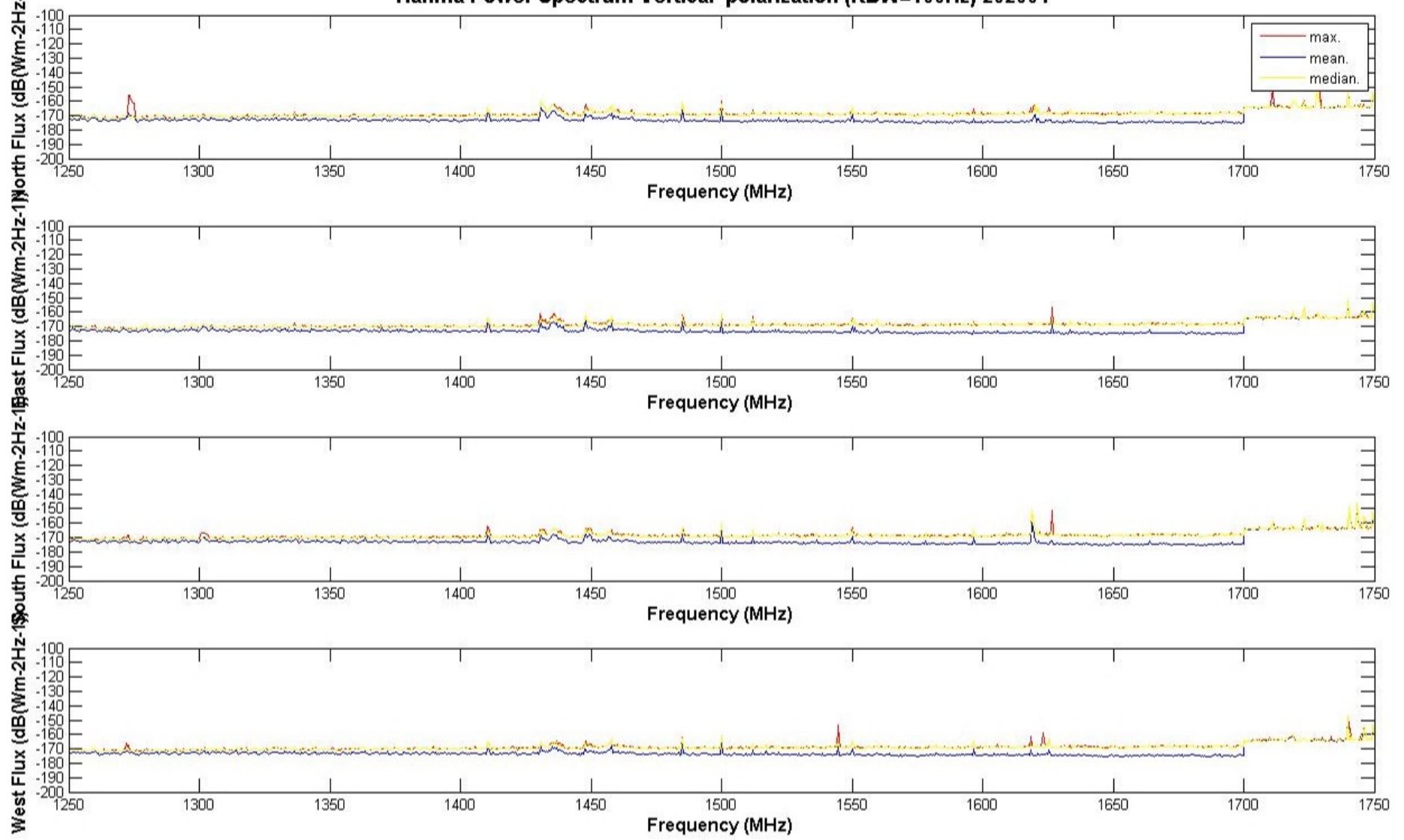
Tianma Power Spectrum Vertical polarization (RBW=100Hz) 202004
