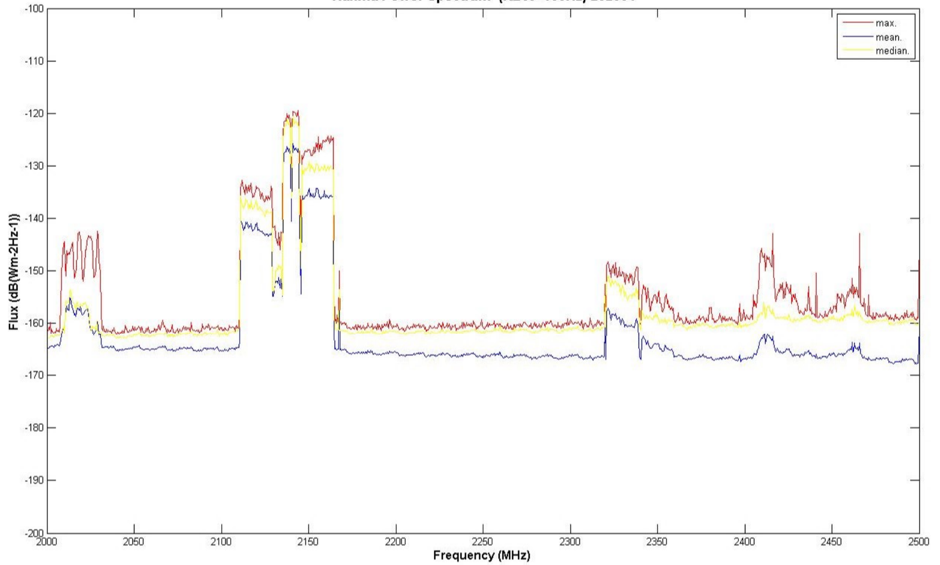
Tianma Power Spectrum (RBW=100Hz) 202004
